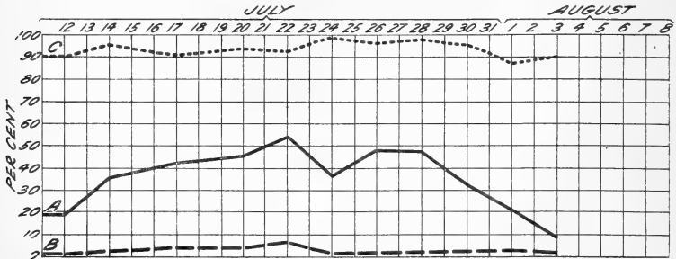
FIG. 8.—Curves showing the percentage of parasitism of Popillia japonica by Centeter cinerea at Koiwai, Japan, during 1921: A, parasitism of female beetles; B, parasitism of male beetles; C, proportion of eggs laid upon female beetles
